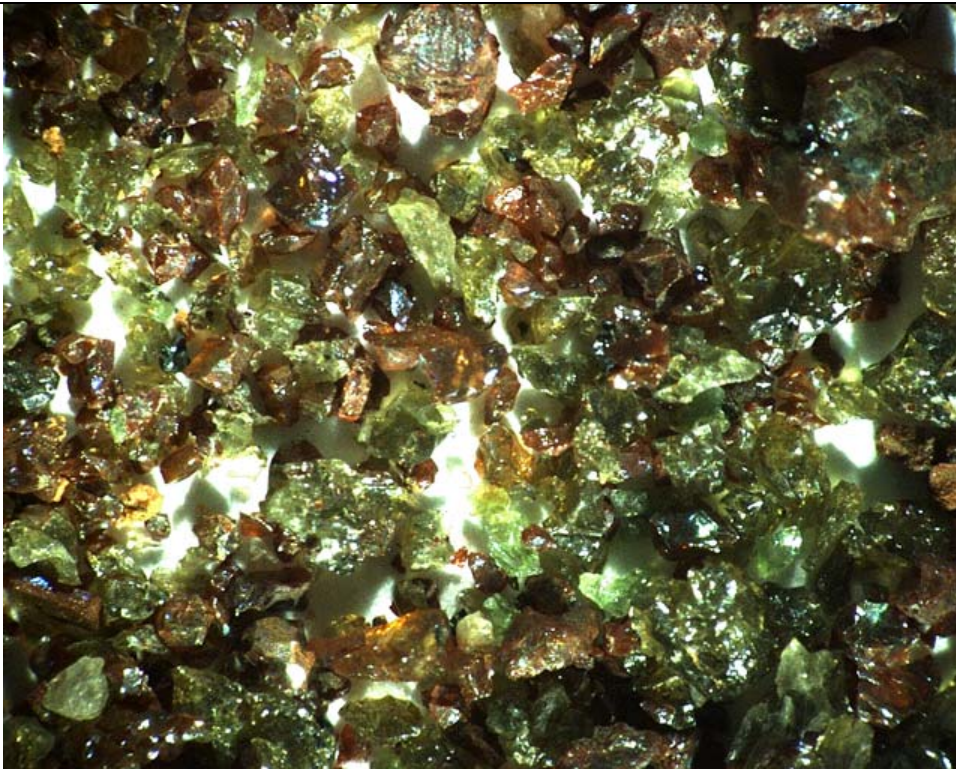
Fired (oxidizing atmosphere) disaggregated xenoliths from Mt. Trumbull, including olivine. Photo by Barbara Bane.
